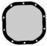
DANA 25,27,30 10 bolt holes 9" wide
